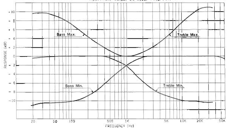
R-3045 Tone Control Input : Aux, Output 8Ω Load, Filter : Off
