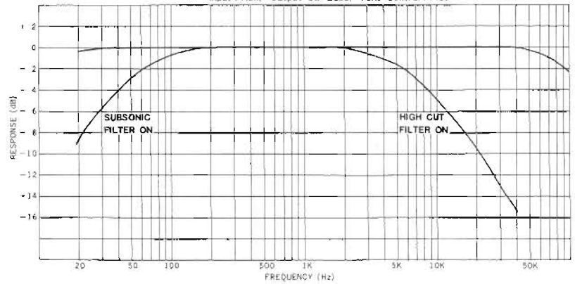
R-3045 Filter Input : Aux, Output 8Ω Load, Tone Control : Flat
