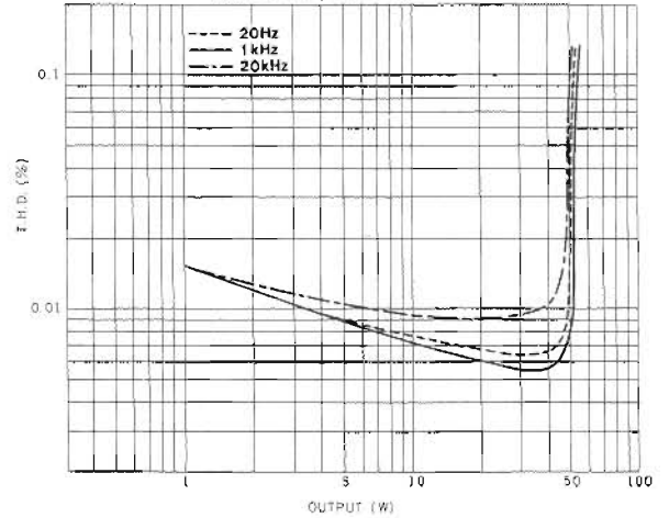
R-3045 T.H. Distortion vs. Power Input : Aux, Output : 8Ω Load Both CH Driven Volume : Max, Tone : Flat
