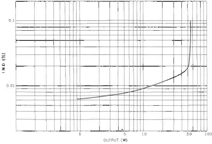
R-3045 I.M. Distortion vs. Power Input : Aux, Output : 8Ω Load Both CH Driven, Volume : Max Tone : Flat, Frequency : 60Hz : 7kHz = 4 : 1
